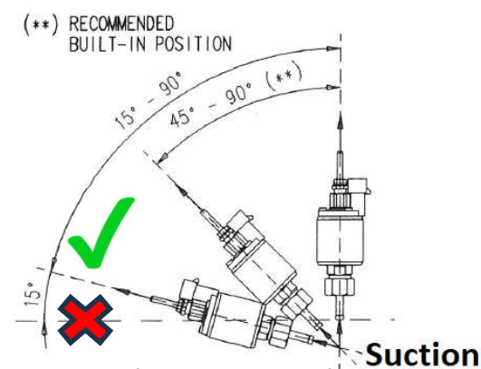
Figur 6 anbefaling installation af pumpe
